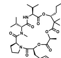
Palmyramide A IC 50 9 nM HCT-119 colon cells
